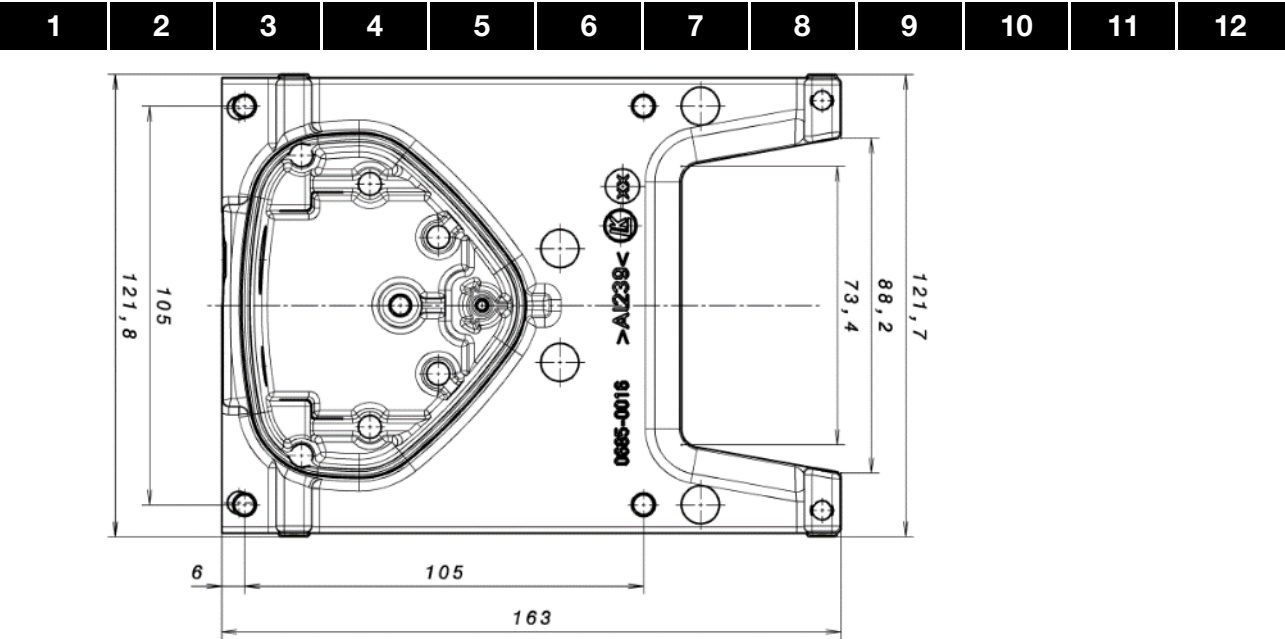
Abb. 63: Bohrbild Standard-Wand-Adapterplatte BG B
