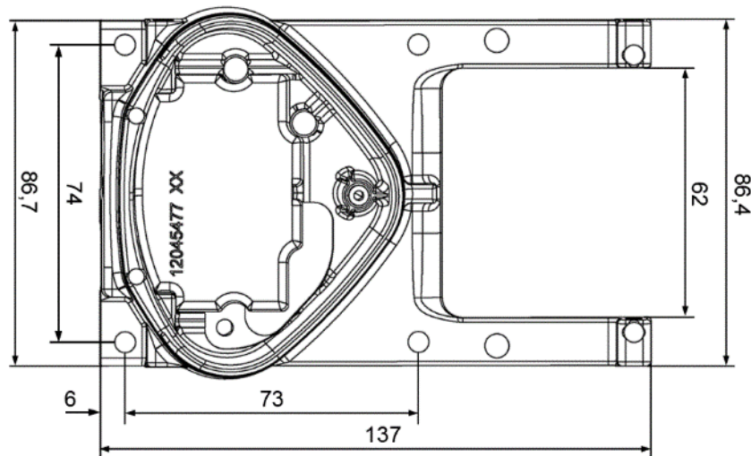
Abb. 62: Bohrbild Standard-Wand-Adapterplatte BG A
