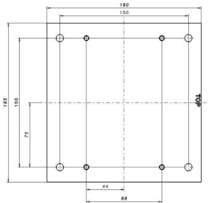
Abb. 65: Bohrbild Standard-Wand-Adapterplatte BG D
