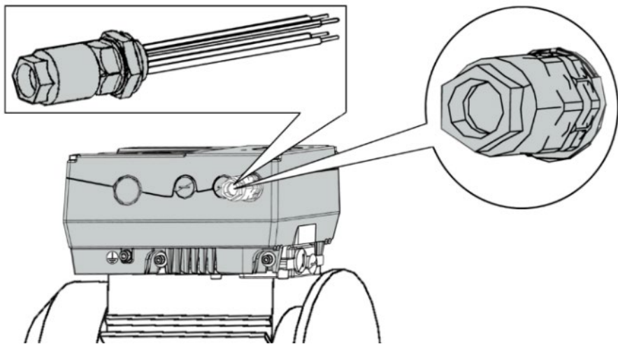
Abb. 20: PHOENIX-Quickon
