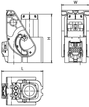
Receptacle Housing
