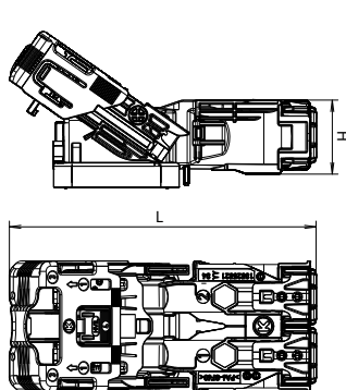
Receptacle Housing
