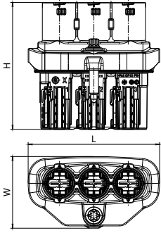
Receptacle Housing
